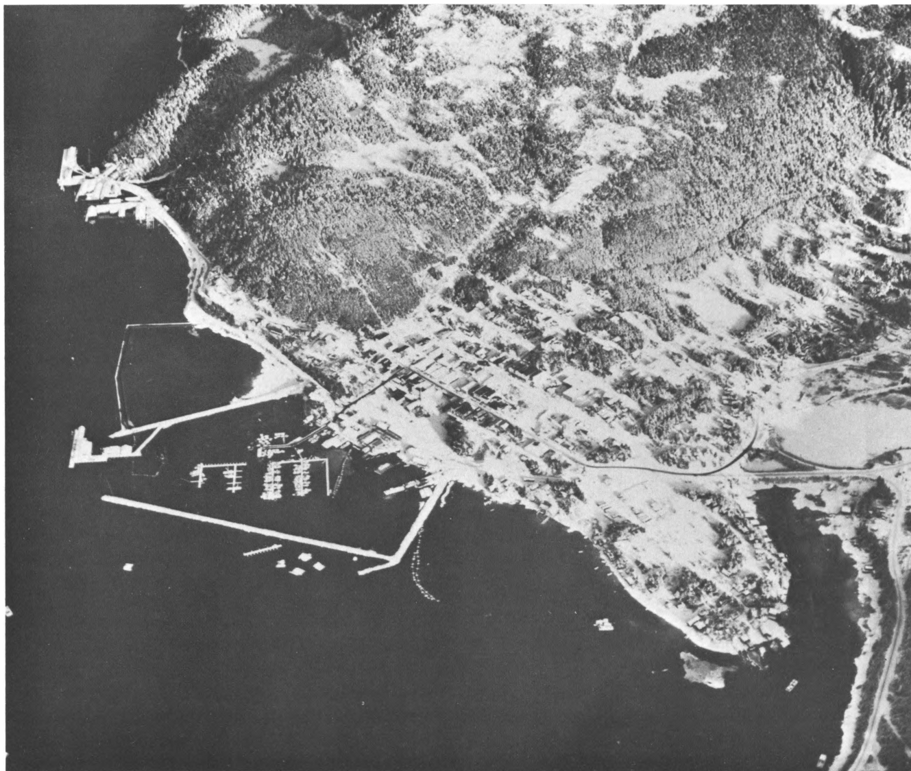
6.—Cordova harbor as it appeared in February 1965. Tectonic uplift left docks inaccessible to ships except at very high tides. Reconstruction involved dredging of harbor and rebuilding of docks and small-boat basin. U. S. Army photograph.
