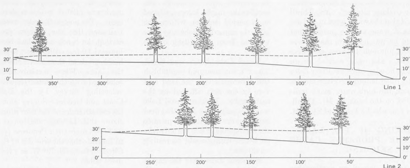
23.—Upper limit of wave damage caused by seiche along two traverses run parallel to wave travel direction on the west side of Ship Creek delta. Locations of traverses are shown on figure 17.
