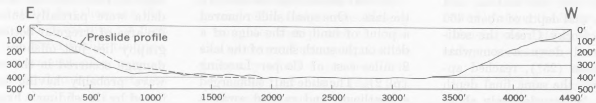
PROFILE ALONG FATHOMETER LINE 89
