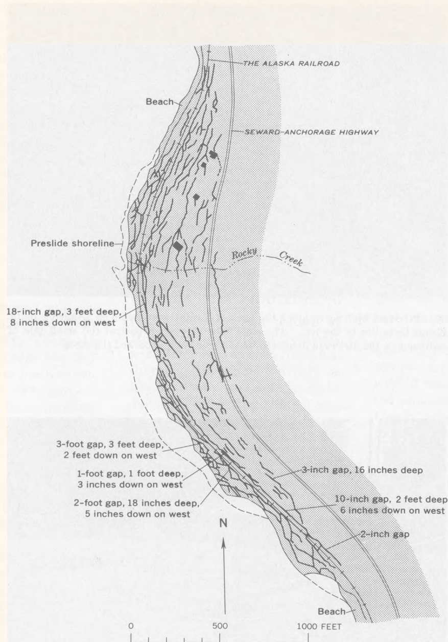
29.—Preslide shoreline, slump scarps, and ground fracturing on Rocky Creek delta.
