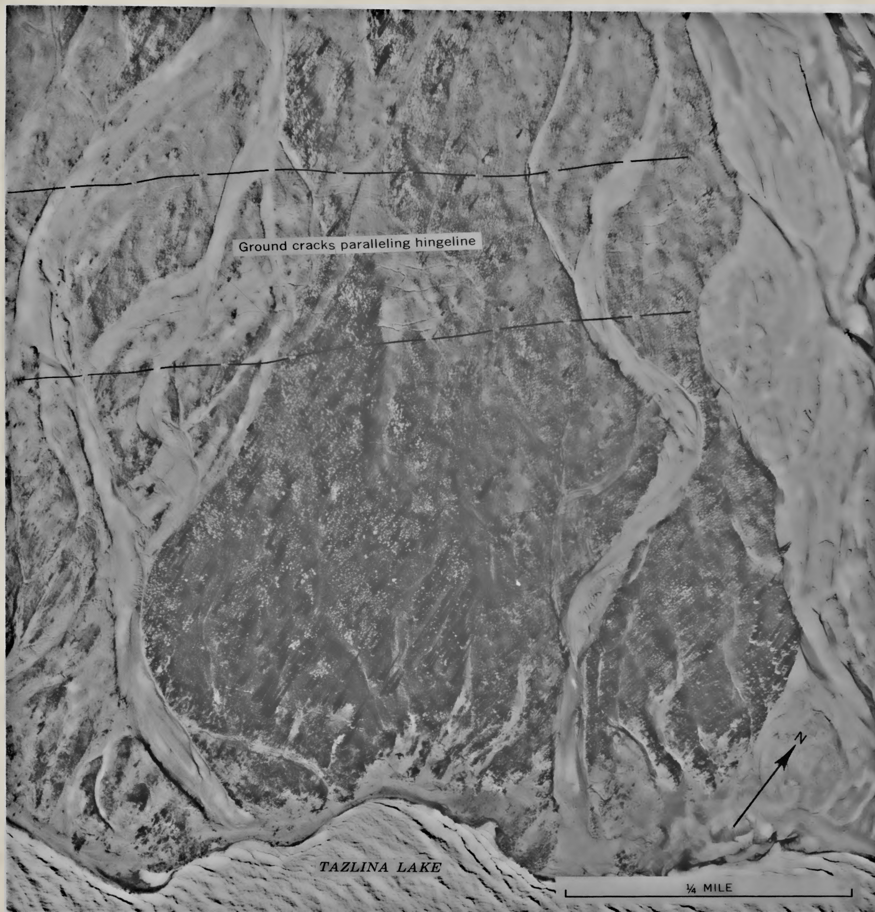
16.—Ground cracks along and paralleling hingeline on Nelchina River delta. Photograph by U.S. Geological Survey, October 1964.
