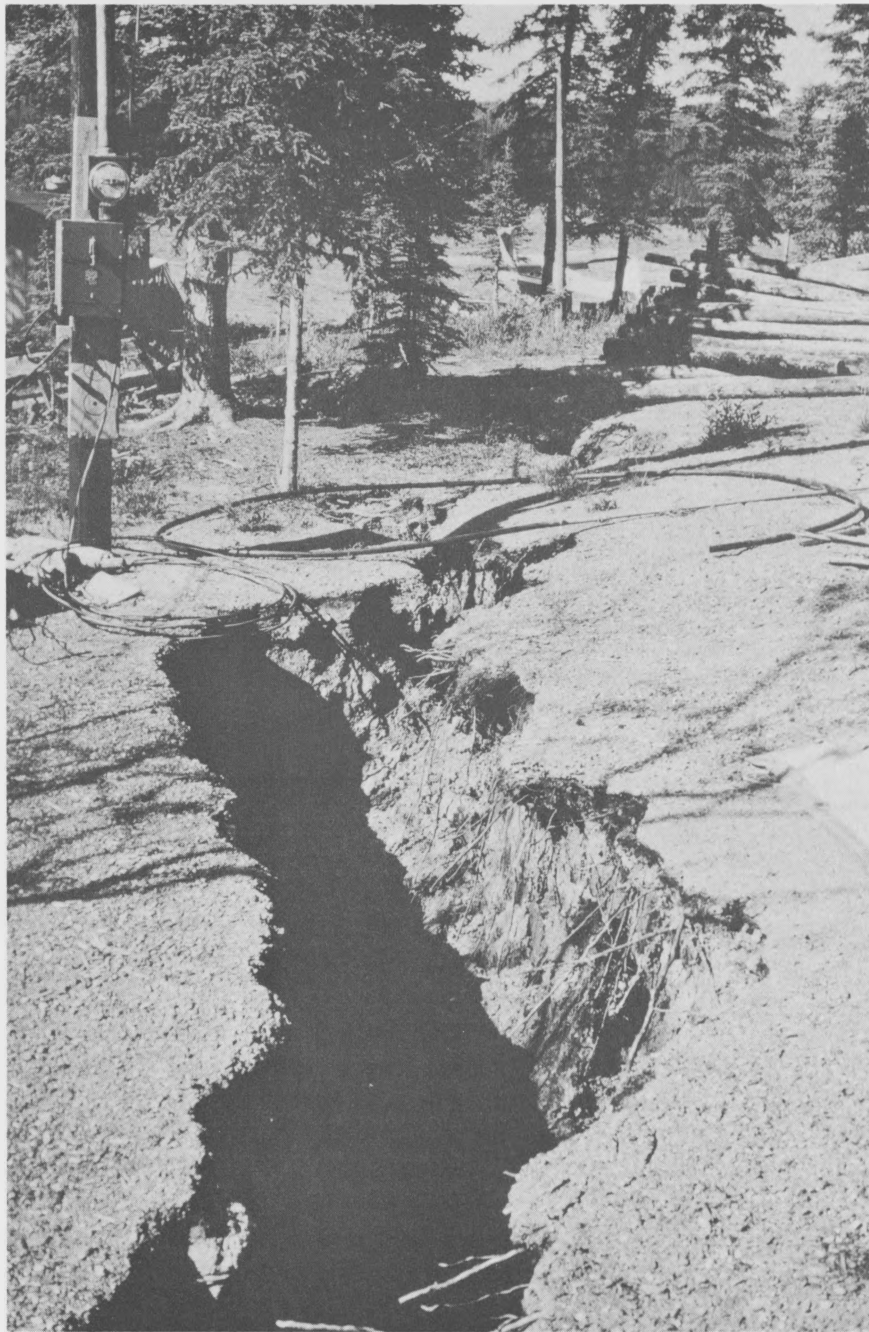
12.—Large ground crack formed in clearing along south shore of lake about two-tenths of a mile north of mile 158, Glenn Highway. Maximum width of crack is 4 feet and depth is 6 feet. This ground crack is one of several that generally parallel the lakeshore.
