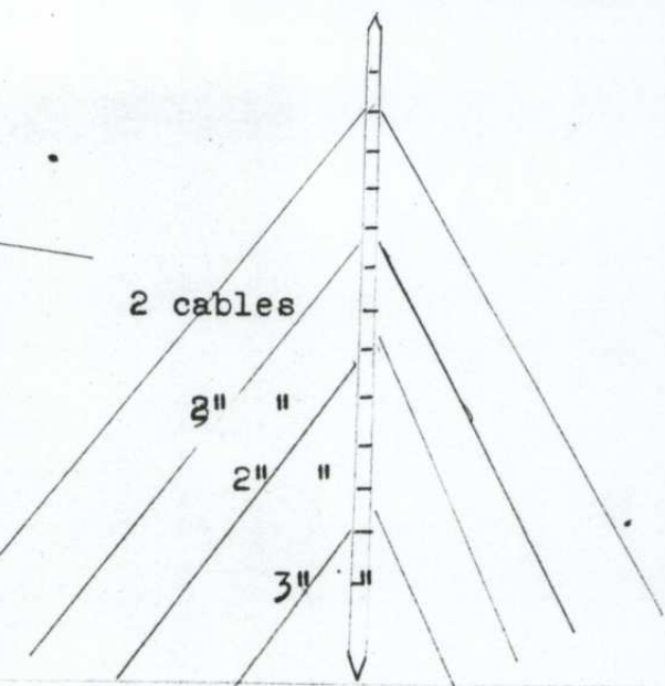
Figure 2. Side view of tower showing 2 of the three wire groups and number of cables in each level.
