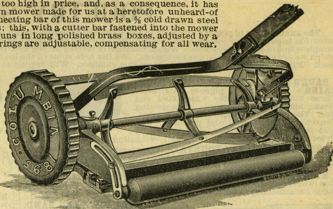
COLUMBIA LAWN MOWER.
